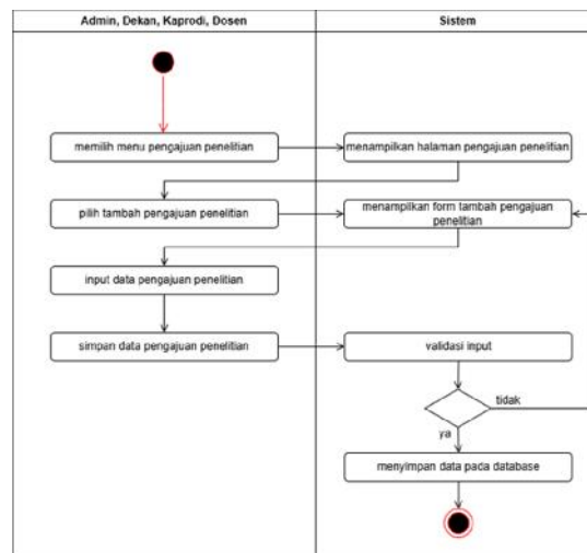
Figure 4. Activity Diagram
