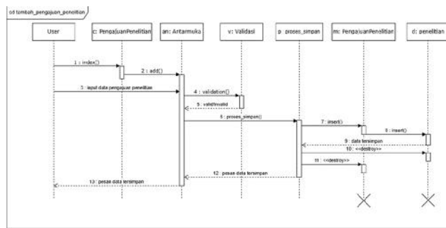
Figure 5. Sequence Diagram
