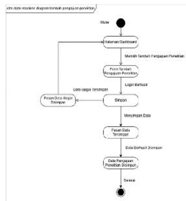
Figure 6. State Machine Diagram
