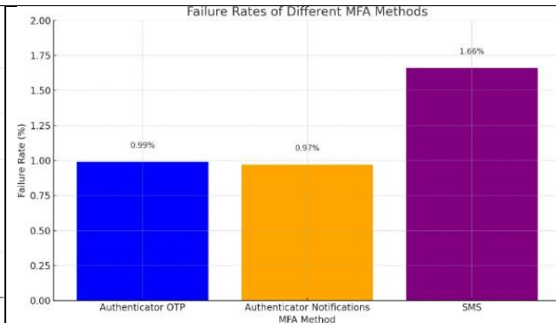
Figure 7: Failure Rates of Different MFA Methods
