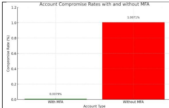
Figure 6: Account compromise rate with and without
