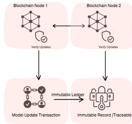
Fig. 3. The federated learning integrated with blockchain: enhanced transparency and traceability.
