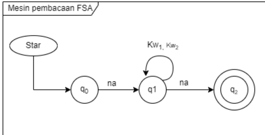
Picture 2. Finite State Automata
